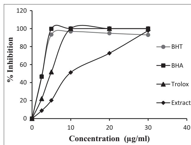
Figure 4: Free radical scavenging activity of different concentrations of the methanol extract and standards by ABTS radicals
